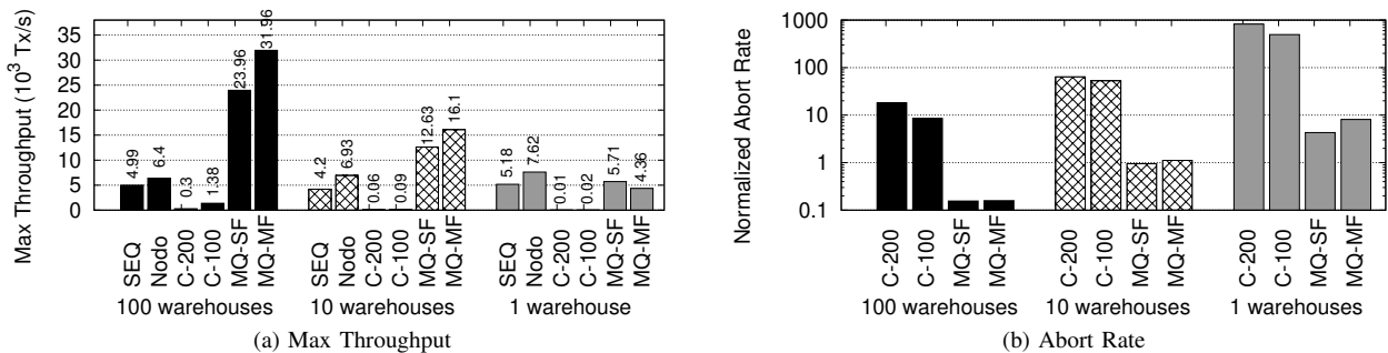
Fig. 3: Maximum sustainable throughput and normalized abort rates for TPC-C benchmark at different levels of contention.
