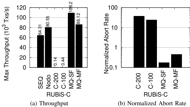
Fig. 4: Maximum sustainable throughput and normalized abort rates for RUBiS benchmark.
