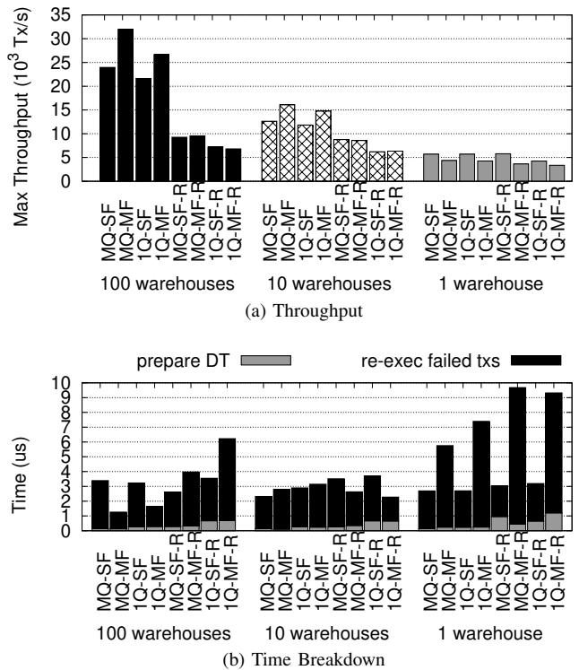
Fig. 5: Maximum sustainable throughput and per transaction execution times for various Prognosticator variants with TPC-C benchmark at different levels of contention.
