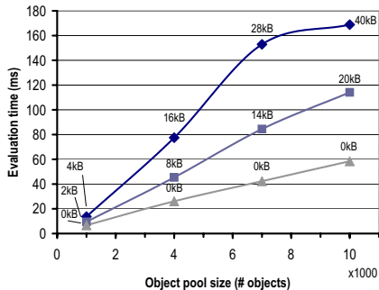
Fig. 11. Evaluation of CMB Version 3 round handler.
