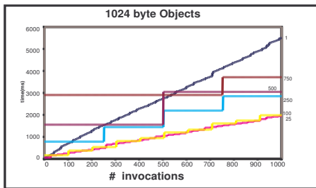
a) Incremental replication without clustering.
