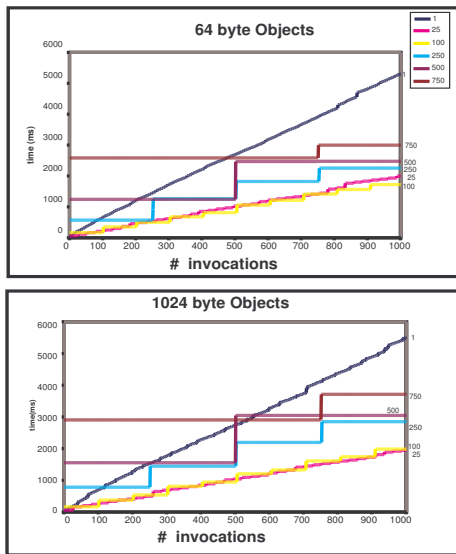
a) Incremental replication without clustering.
