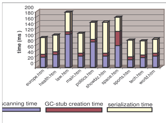
d) Time spent for the top group.
