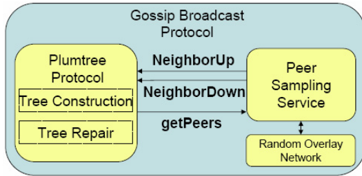
Figure 1. Plumtree architecture
