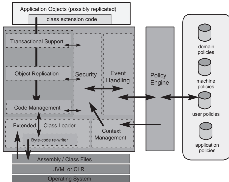
Figure 1: PoliPer architecture. Transactions, replication and code relocation are policy-driven. Policies are enforced and mediated through event-handling. Security module validates every action performed.
