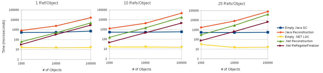
Figure 6: Total LGC Overhead due to Enforcement of the Union Rule
