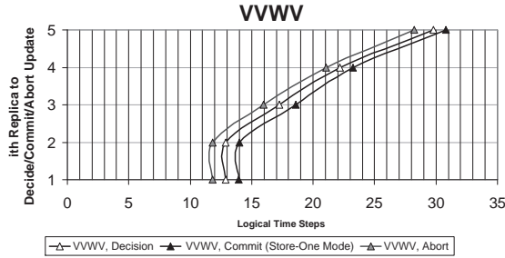
Fig. 3. Average decision vs. commitment vs. abort delays for VVWV in a high-contention scenario. 41 Partitions, mobProb=25\% , updProb=\frac{0.9\%}{5} = 0.18\% .
