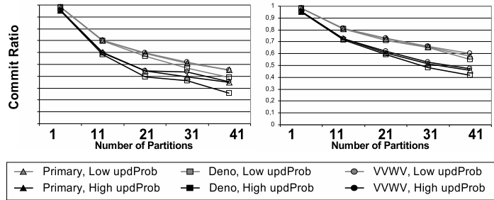
Fig. 1. commit ratios vs. number of partitions. Both low and high site mobility are considered (resp., mobProb=25\% and mobProb=75\% ); and both low and high update probabilities are considered (resp., updProb=\frac{0.5\%}{5} and updProb=\frac{0.9\%}{5} ).
