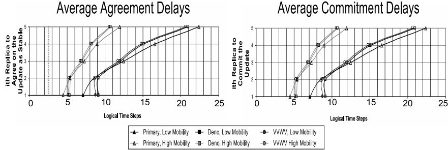
Fig. 2. Average agreement delays, for low site mobility ( mobProb=25\% ) and high site mobility ( mobProb=75\% ), updProb=\frac{0.5\%}{5} = 0.1\% and 11 Partitions.
