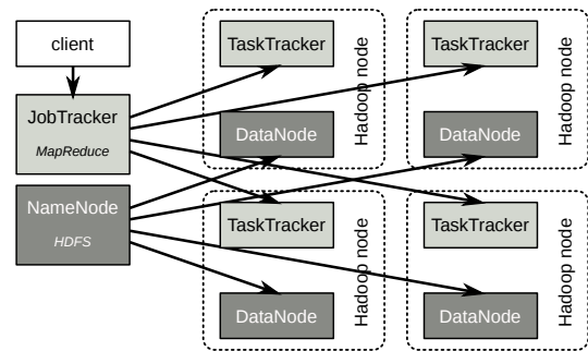
Fig. 1: Hadoop architecture.
