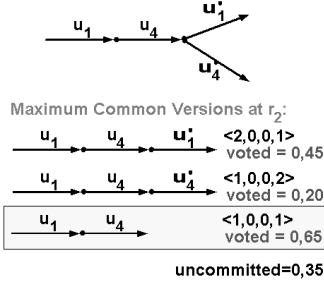
Figure 2: Election decision for replica r_2 at the final state in Figure 1. Among the potential maximum common versions, obtained from the candidates known by r_2 , candidate \langle 1, 0, 0, 1 \rangle is found to have collected a plurality of votes and, thus, updates u_1 and u_4 will be committed in that order.
