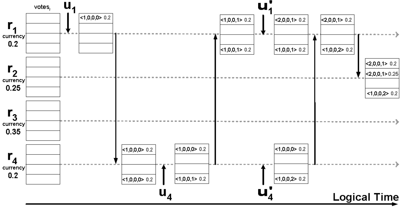
Figure 1: Example of update generation and propagation through anti-entropy sessions, using tentative view. Four replicas of the same logical object, r_1 , r_2 , r_3 and r_4 , start from a common initial stable version, \langle 0, 0, 0, 0 \rangle and currency is unevenly divided among the replicas.
