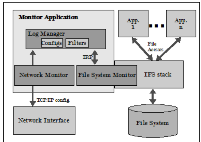
Figure 1: Overview of the File Access Monitor.
