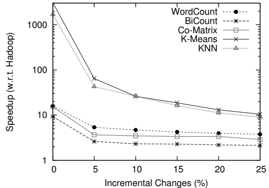
Figure 5: Work speedups versus change size.
