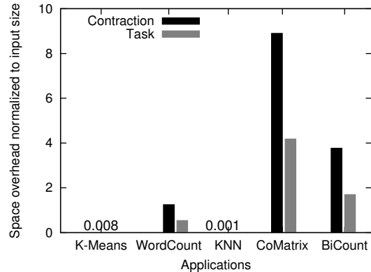
(b) Space overhead
