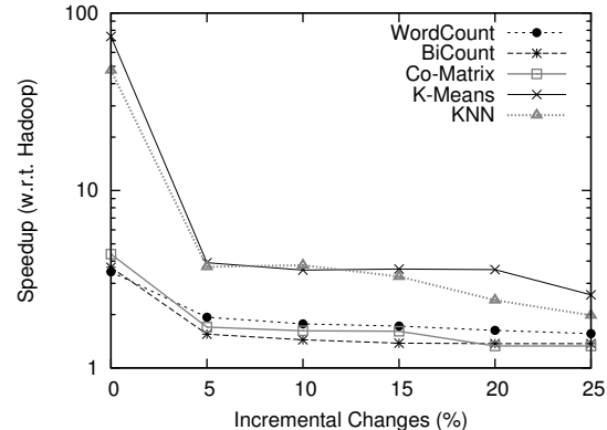
Figure 6: Time speedups versus change size.
