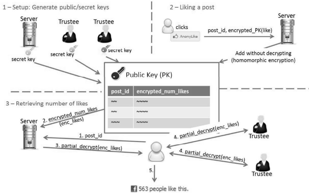
Fig. 1. The 3 steps of the AnonyLikes protocol
