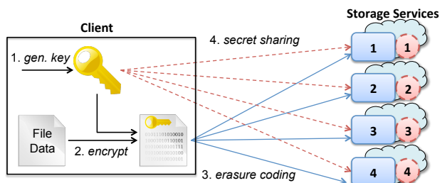
Figure 6: A write in SCFS using the DepSky protocols.
