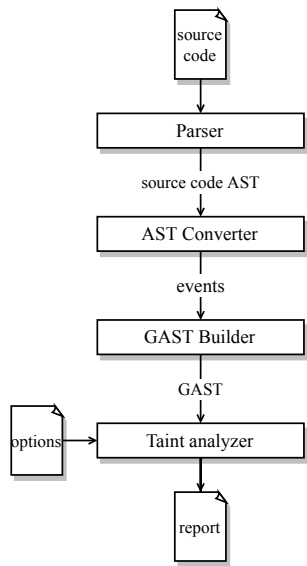
Fig. 1. The GT tool data flow and architecture
