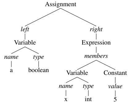
Fig. 2. GAST resulting from executing Listing 5
