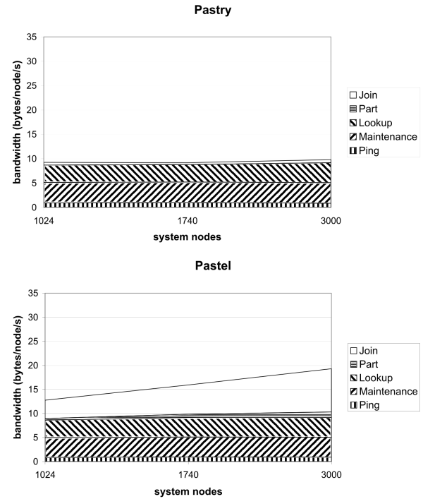
Figure 2. Bandwidth of Pastry and Pastel, with b = 3 , L = 8 and k = 5 ( T = 1 h)
