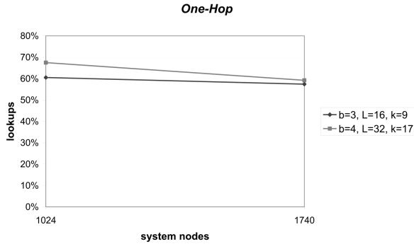
Figure 6. Percentage of lookups satisfied in one hop, with L = 2^{b+1} and k = L/2 + 1 ( T = 1h )
