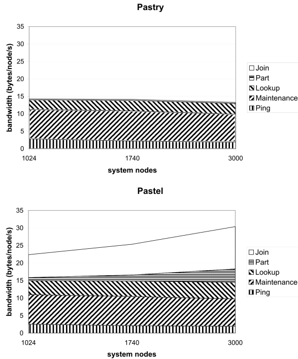
Figure 1. Bandwidth of Pastry and Pastel, with b = 4 , L = 16 and k = 9 ( T = 1 h)
